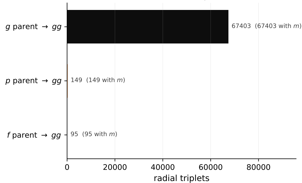
(a) parametric: one parent \rightarrow two daughters 67647 radial triplets
