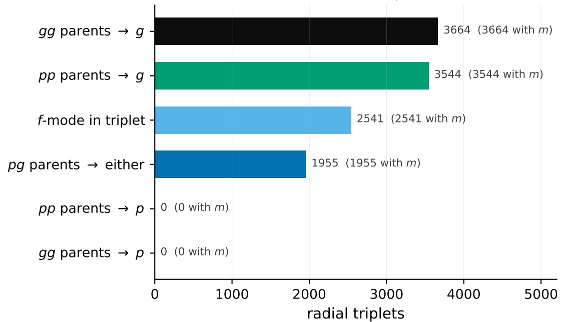
(b) direct: two parents \rightarrow one daughter 11704 radial triplets
