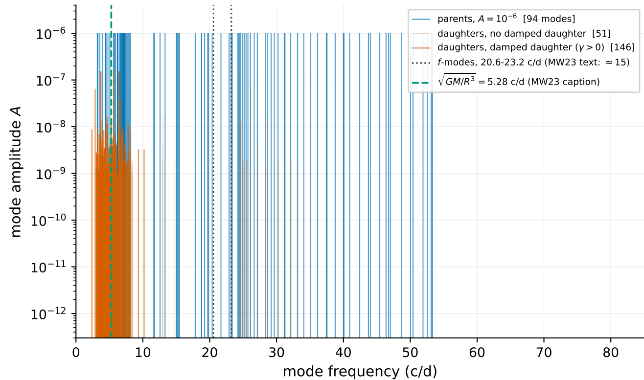
MW23 Fig. 6: 197 triplets with \mu > 10^3 ; A_c = \mu A_a A_b at A_a = A_b = 10^{-6}
