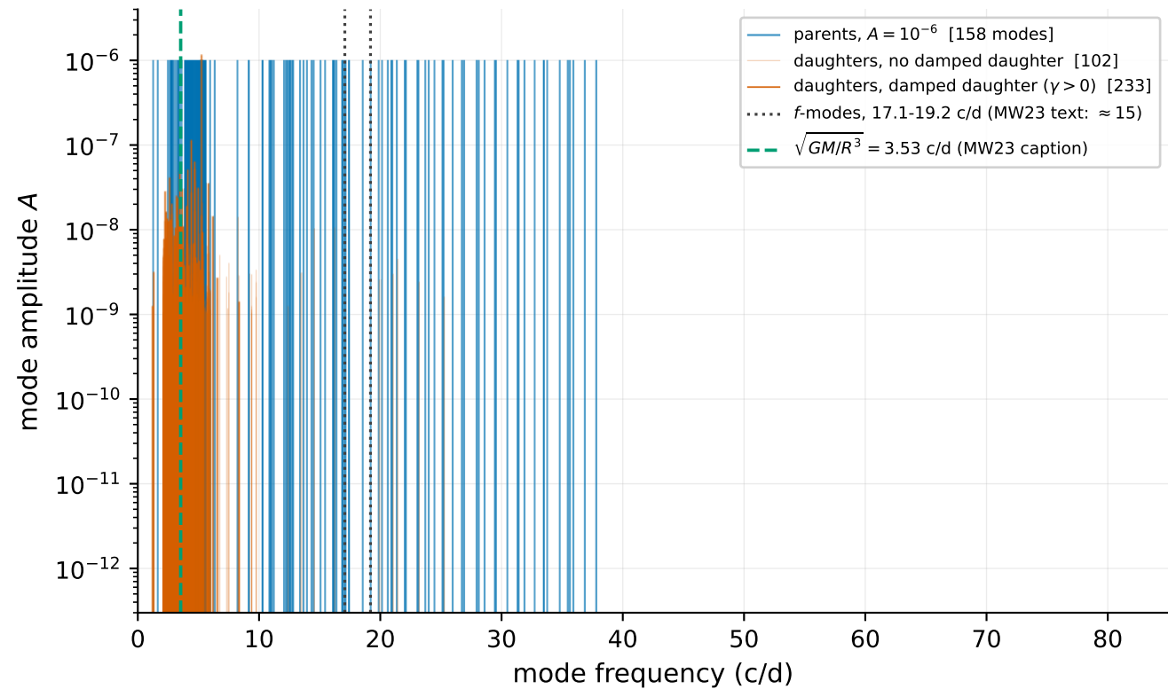
MW23 Fig. 6: 335 triplets with \mu > 10^3 ; A_c = \mu A_a A_b at A_a = A_b = 10^{-6}
