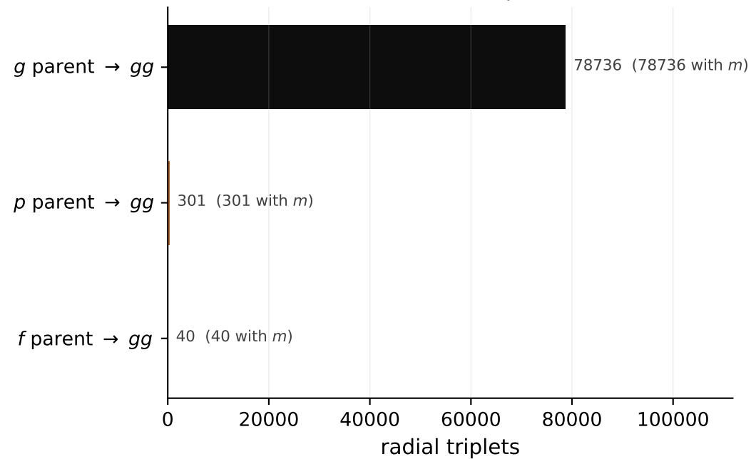
(a) parametric: one parent \rightarrow two daughters 79077 radial triplets
