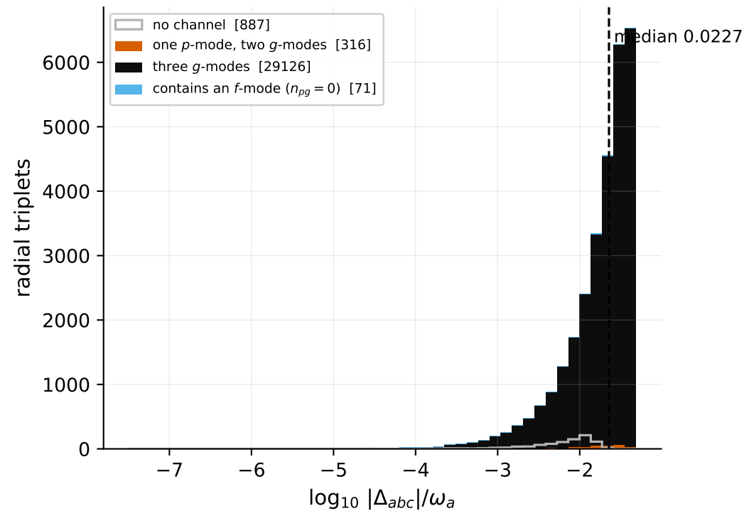
(a) 29513 parametric radial triplets by p/g make-up
