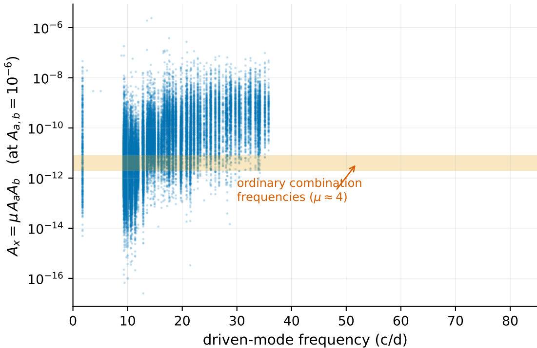
Predicted three-mode amplitudes, all 71142 triplets
