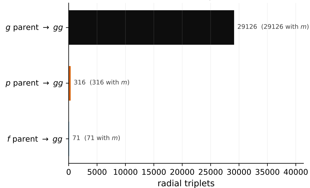
(a) parametric: one parent \rightarrow two daughters 29513 radial triplets
