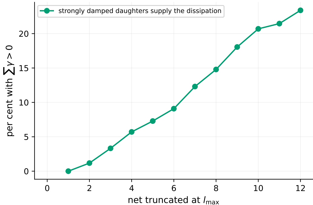
(c) triplets that can reach an equilibrium at all
