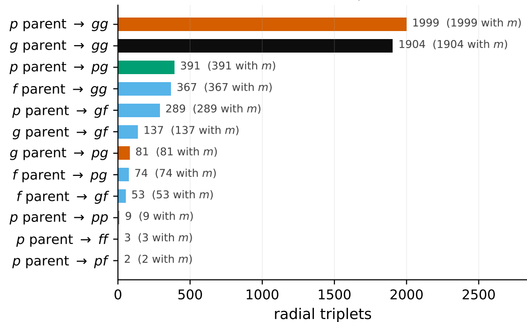
(a) parametric: one parent \rightarrow two daughters 5309 radial triplets
