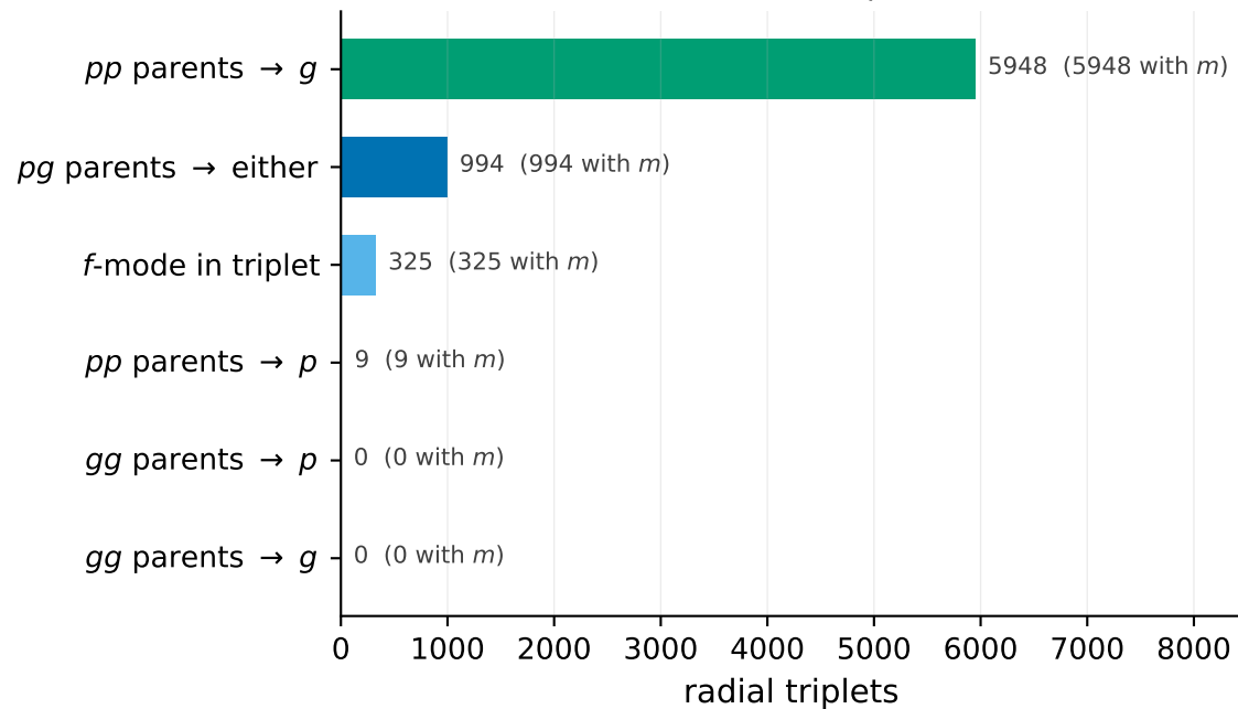
(b) direct: two parents \rightarrow one daughter 7276 radial triplets
