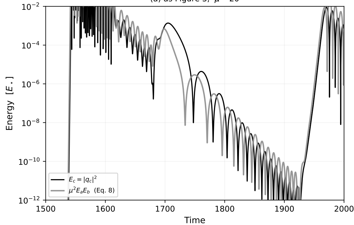
(a) as Figure 3, \mu = 20
