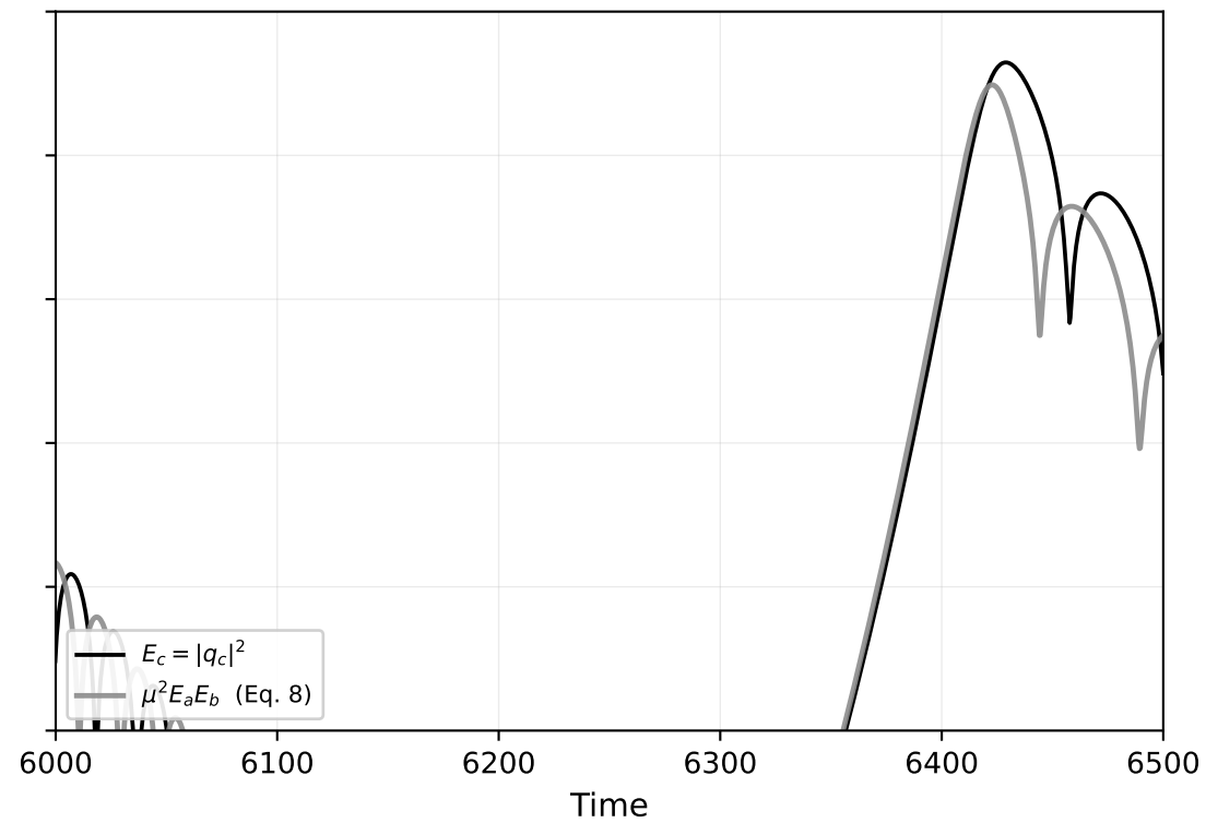
(b) parent driving \times 0.3 , \mu = 20
