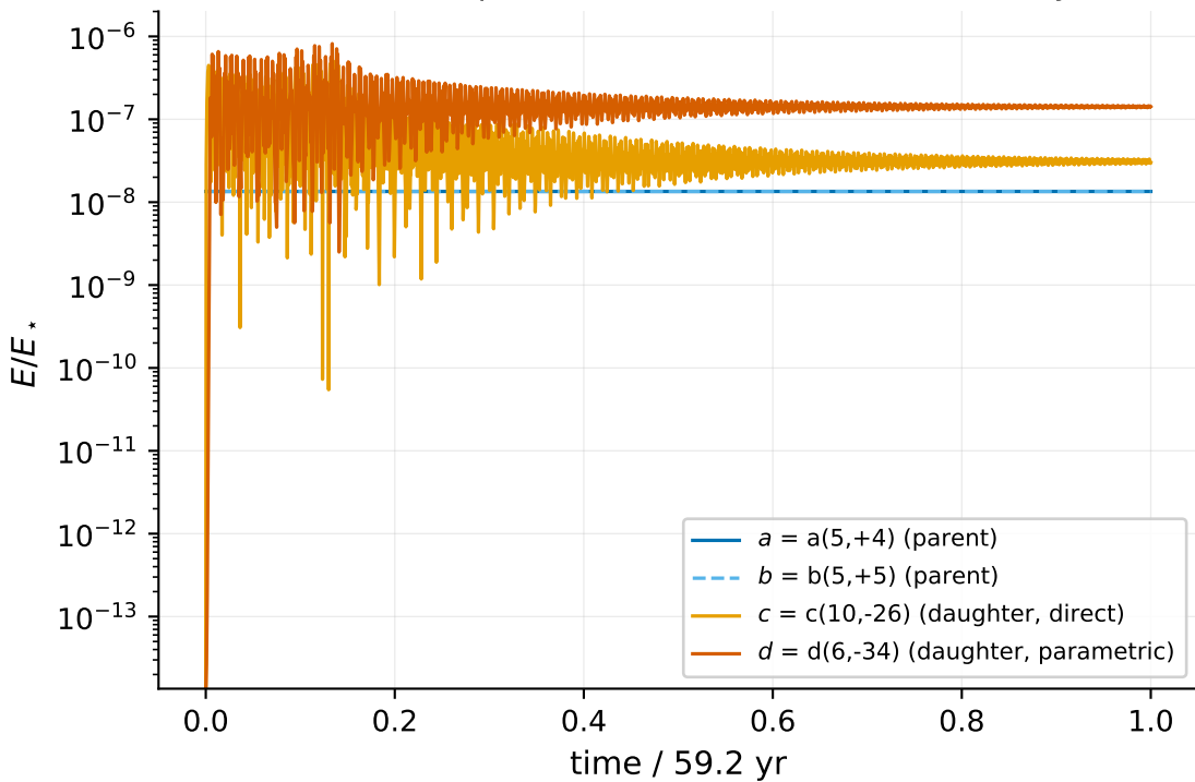
Mixed direct/parametric network, 4 modes, 59.2 yr
