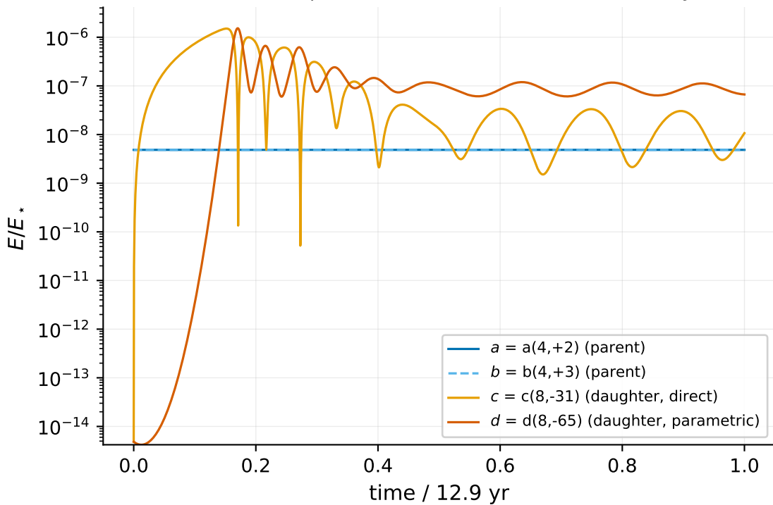
Mixed direct/parametric network, 4 modes, 12.9 yr
