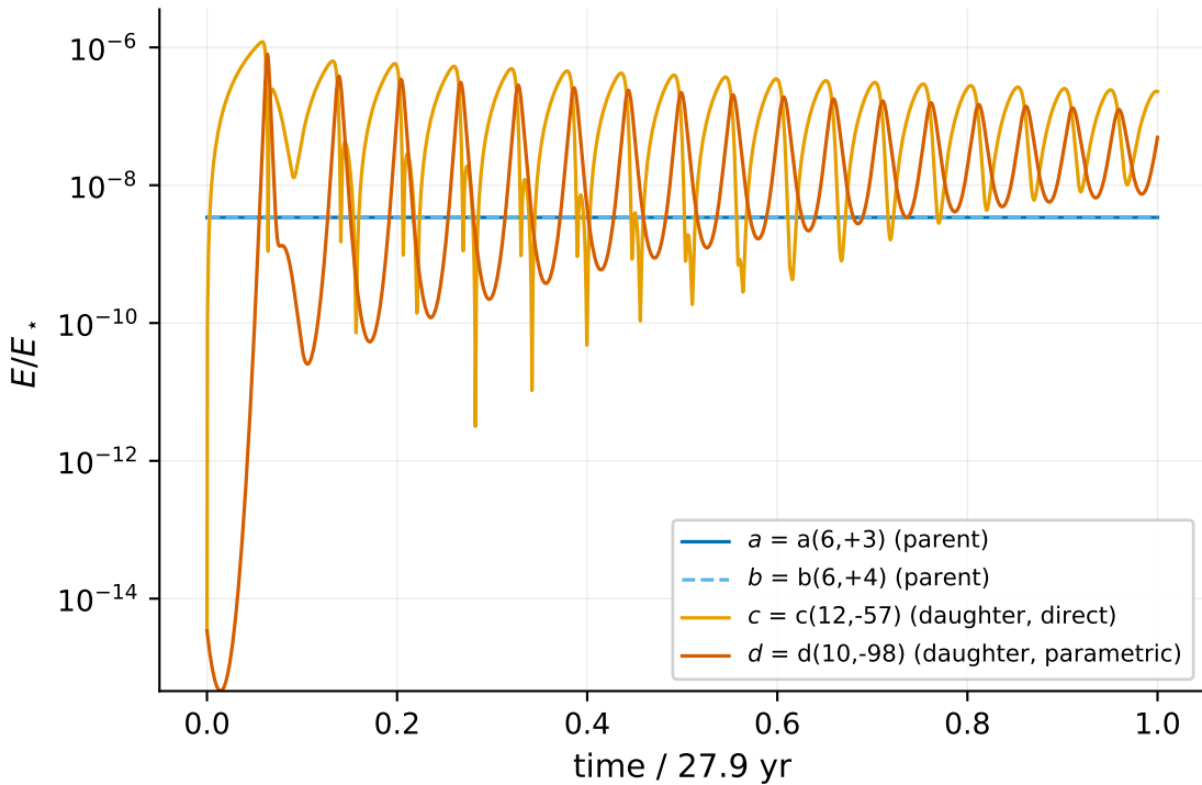
Mixed direct/parametric network, 4 modes, 27.9 yr
