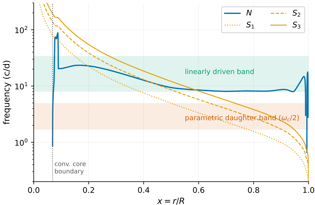
Propagation diagram, M = 2.00 M_{\odot} \delta Sct model
