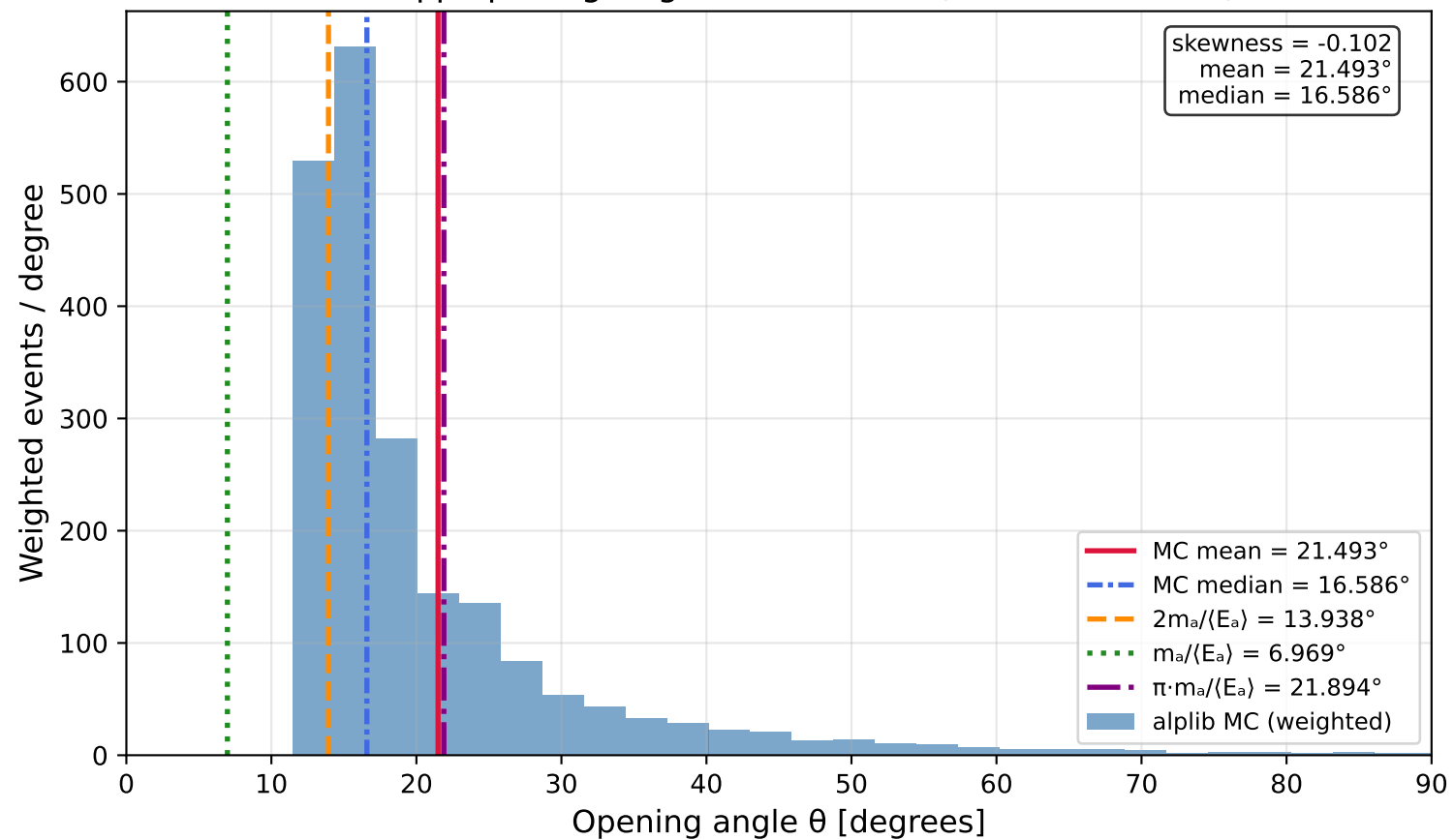
ALP \rightarrow\gamma\gamma Opening Angle Distribution ( m_a = 100.0 MeV)
