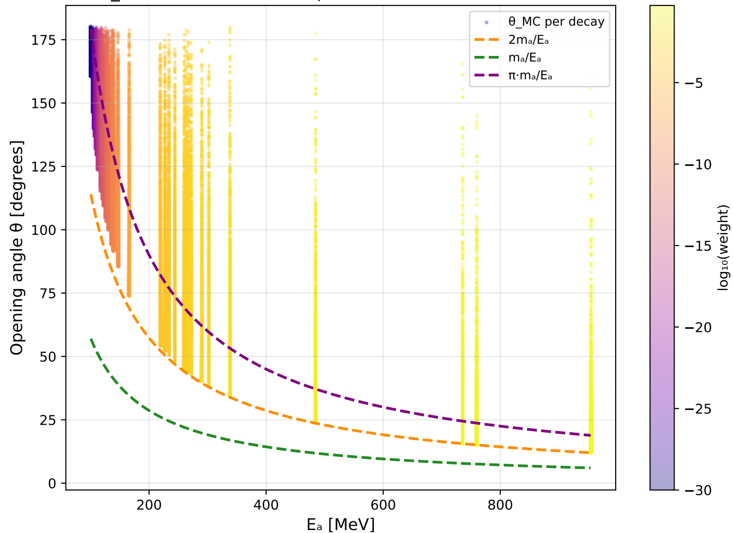
\theta_{MC} vs E_a with formula predictions ( m_a = 100.0 MeV)
