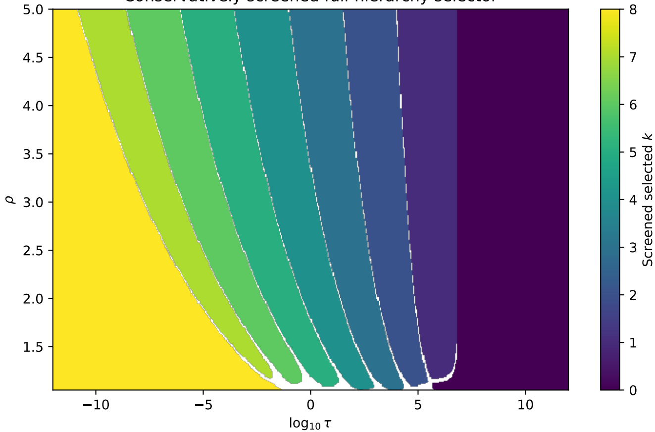
Conservatively screened full-hierarchy selector
