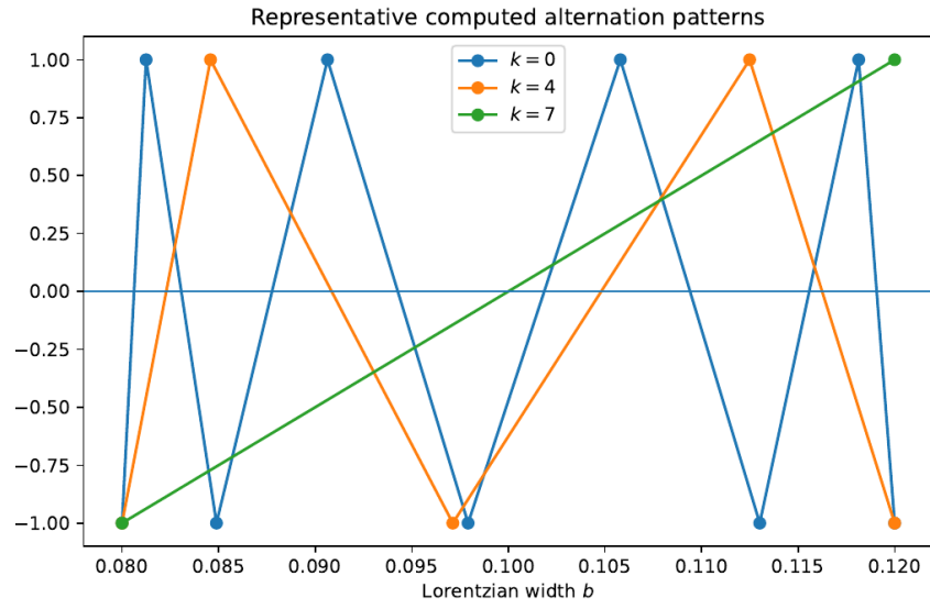
Figure 2: Representative normalized computed alternation patterns from the lower endpoint ( k = 0 ), midpoint ( k = 4 ), and upper half ( k = 7 ) of the n = 4 hierarchy.
