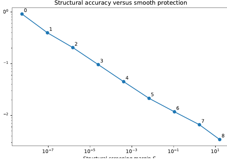
Figure 3: Each added moment decreases the smooth-risk norm but increases the Lorentzian structural error. Labels indicate the moment depth k .
