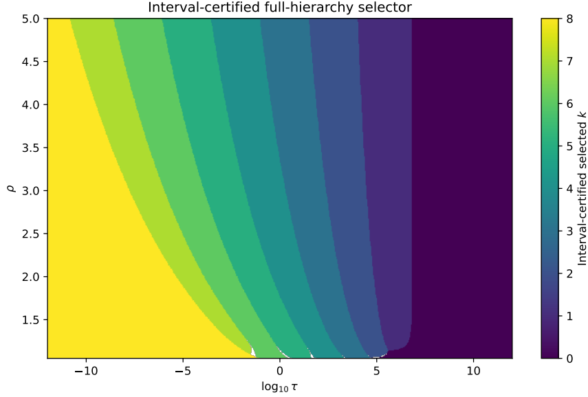
Figure 4: Interval-certified full-hierarchy selector. Blank regions remain unresolved because candidate risk intervals overlap.
