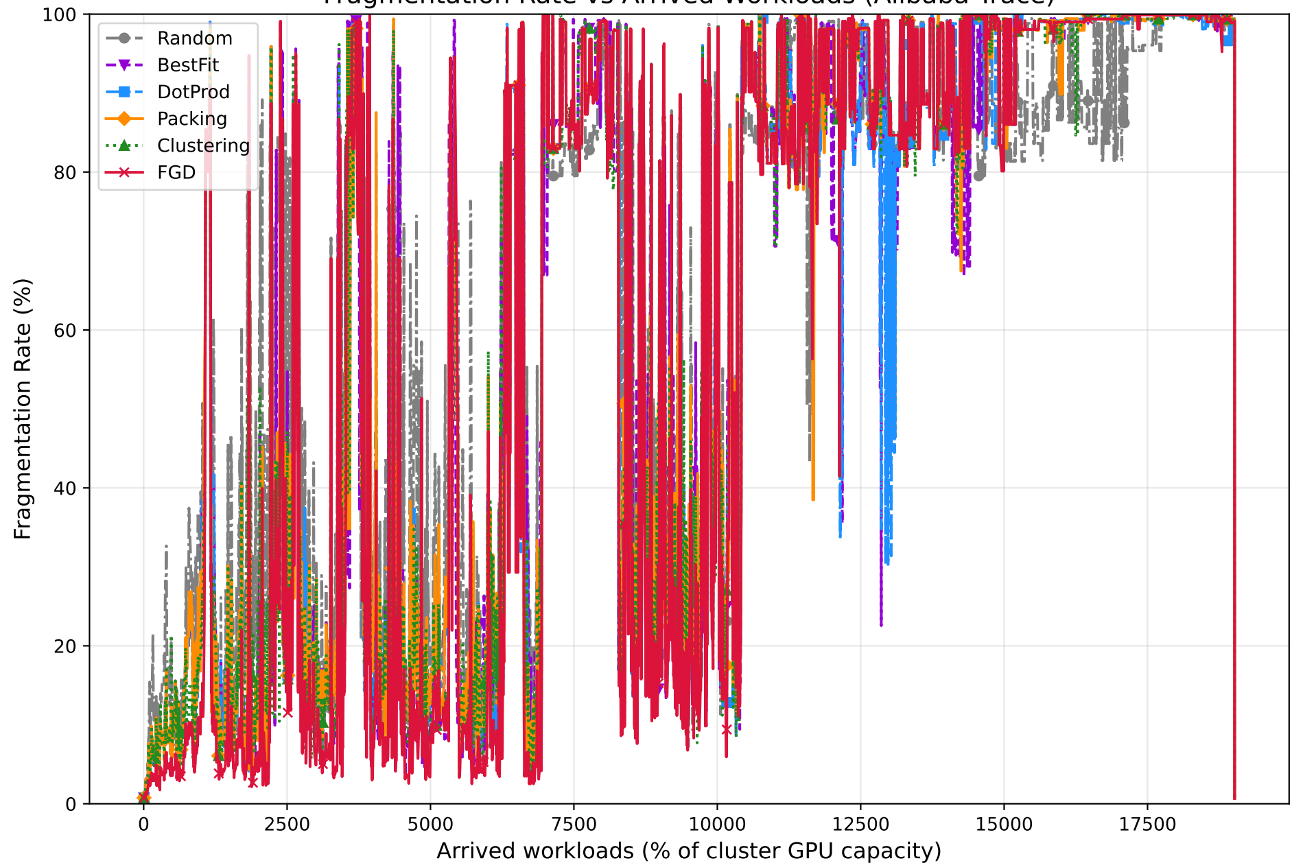
Fragmentation Rate vs Arrived Workloads (Alibaba Trace)
