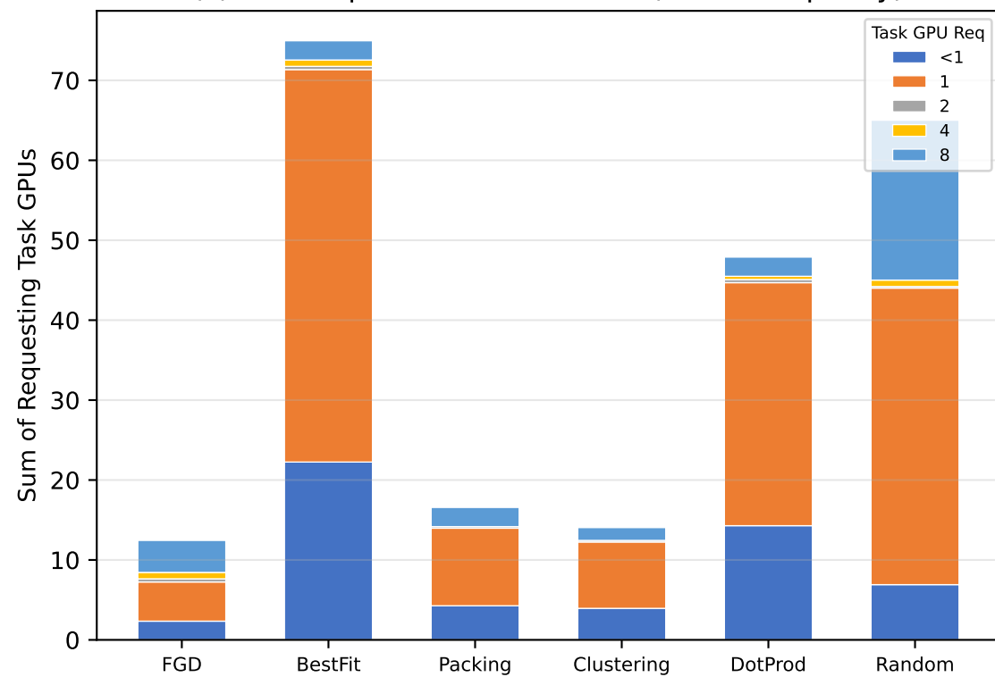
(c) GPU requests of failed tasks (at 96% capacity)
