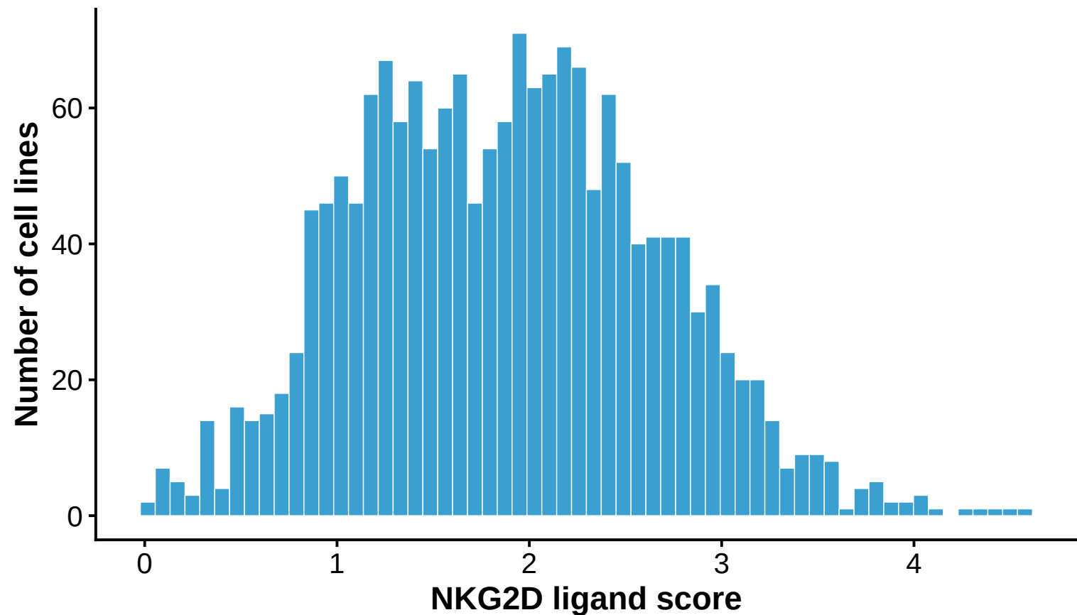
Distribution of NKG2D ligand score across DepMap cell lines
