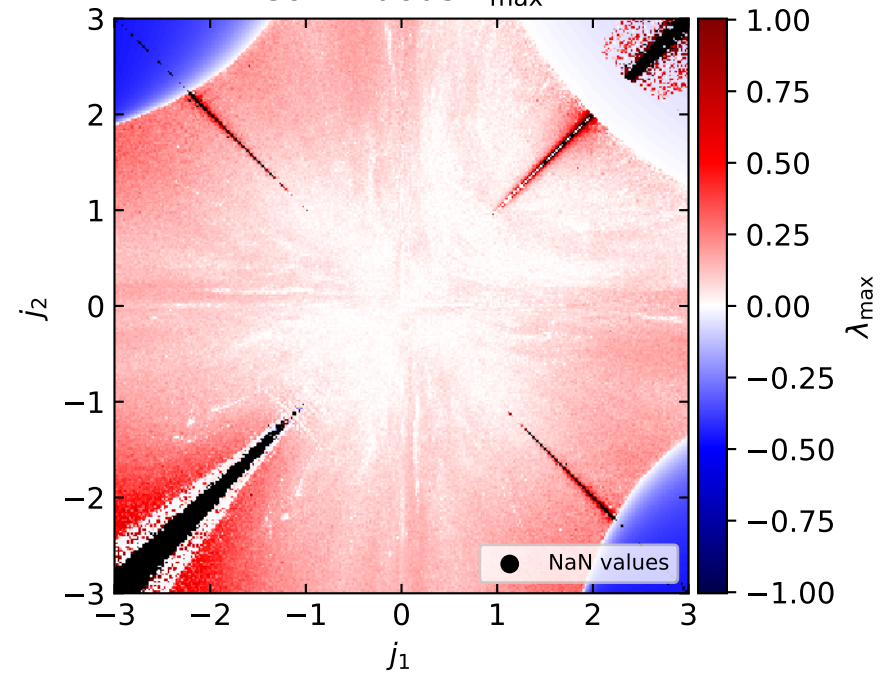
Continuous \lambda_{\max}
