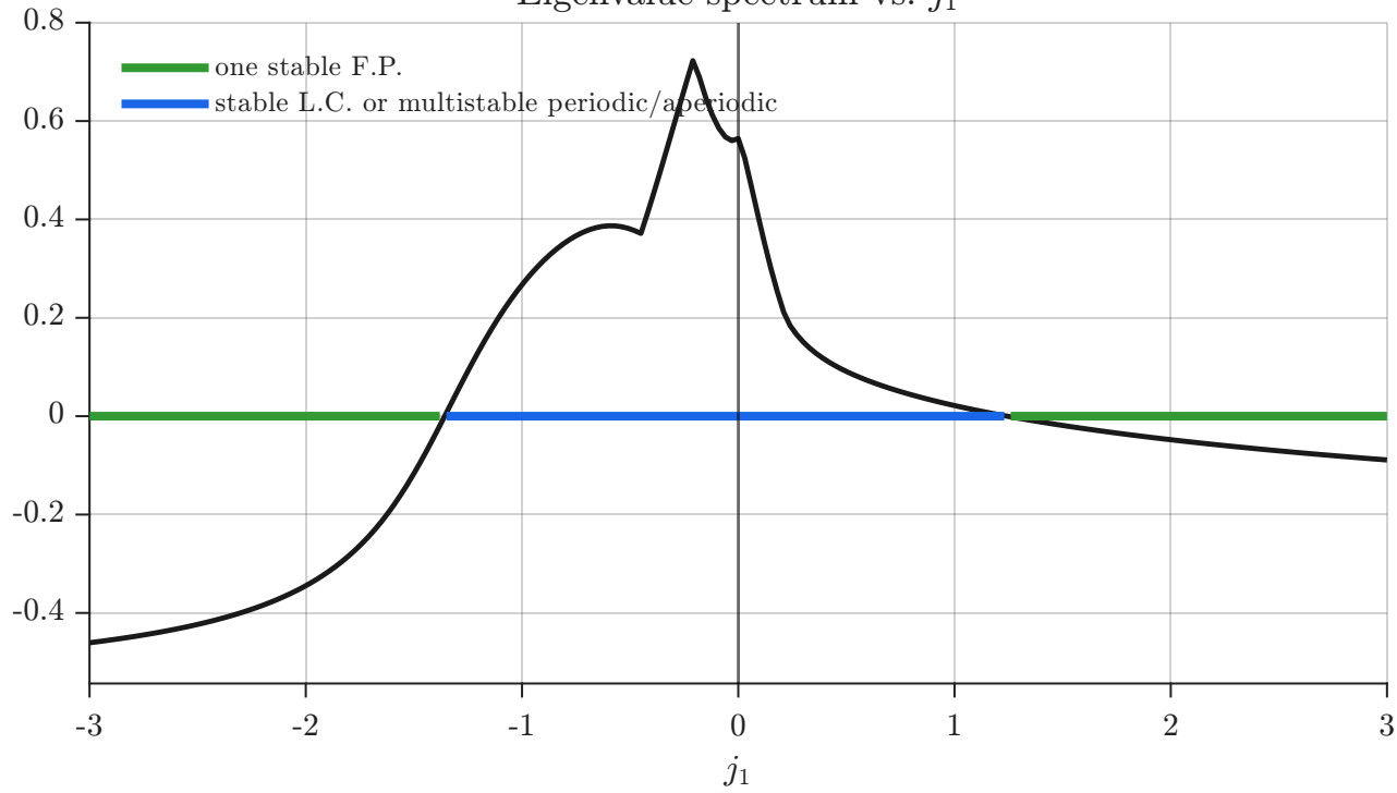
Eigenvalue spectrum vs. j_1
