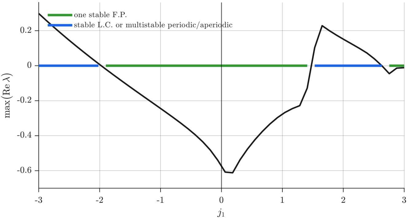
Eigenvalue spectrum vs. j_1
