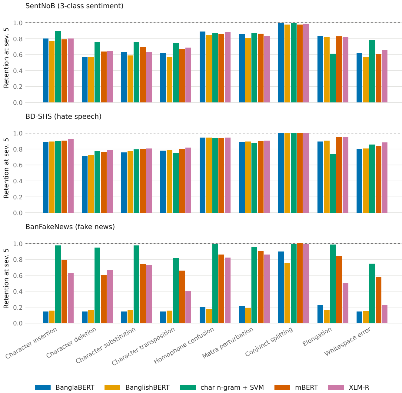
Fraction of clean macro-F1 retained at maximum noise severity 1.0 = no degradation. Mean over 3 seeds.
