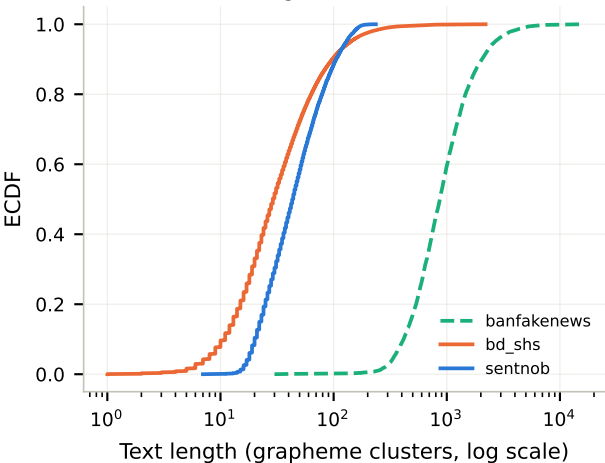
Length ECDF (raw)
