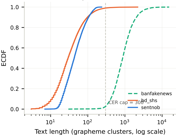
Length ECDF (final)
