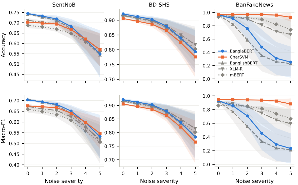
Degradation under synthetic orthographic/typographic noise (mean \pm 1 SD over 3 seeds; clean = severity 0)
