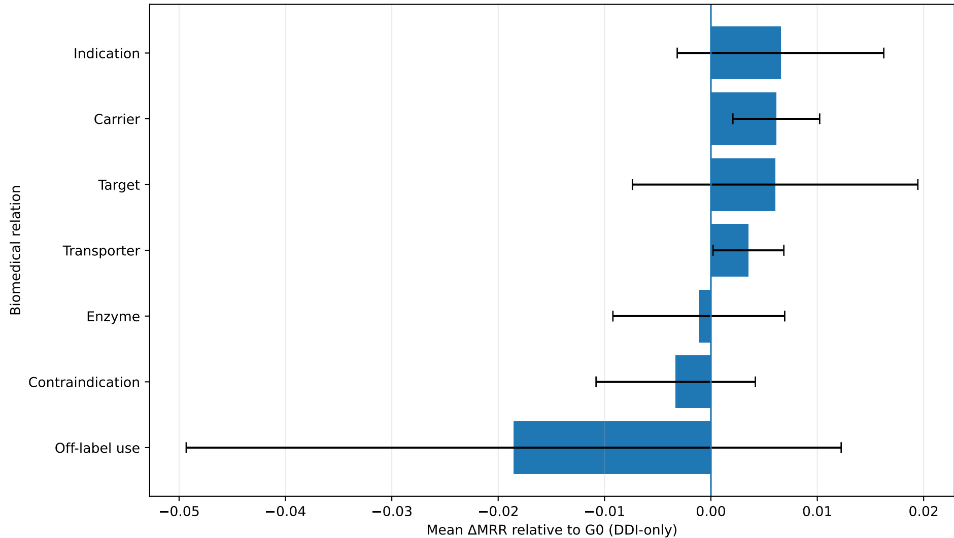
Relation-Level Ablation: Effect of Biomedical Relations on DDI Prediction
