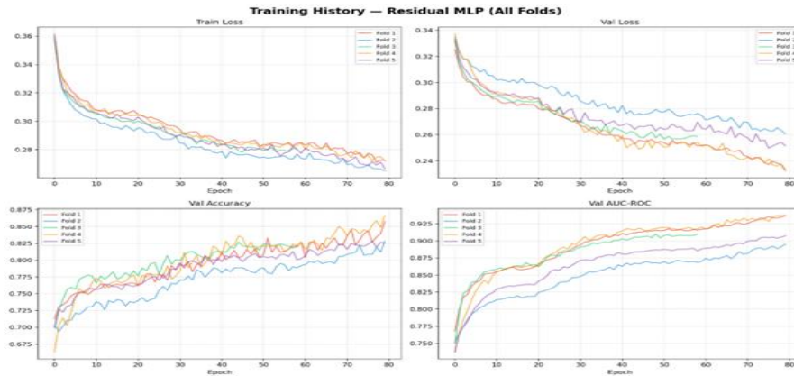
Figure 6.1: Training History — Residual MLP (All 5 Folds): Train/Val Loss, Validation Accuracy, and Validation AUC-ROC
