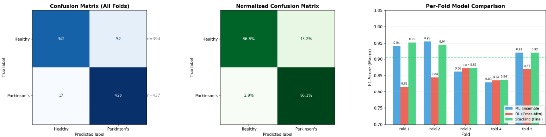
Figure 6.6 Speech confusion matrix (all folds) + normalized CM + per-fold ML vs DL vs Stacking F1
