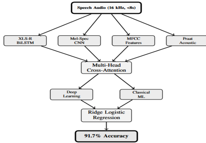
Figure 4.2.2: Speech analysis module with multi-feature pathways and cross-attention fusion achieving 91.7% accuracy.
