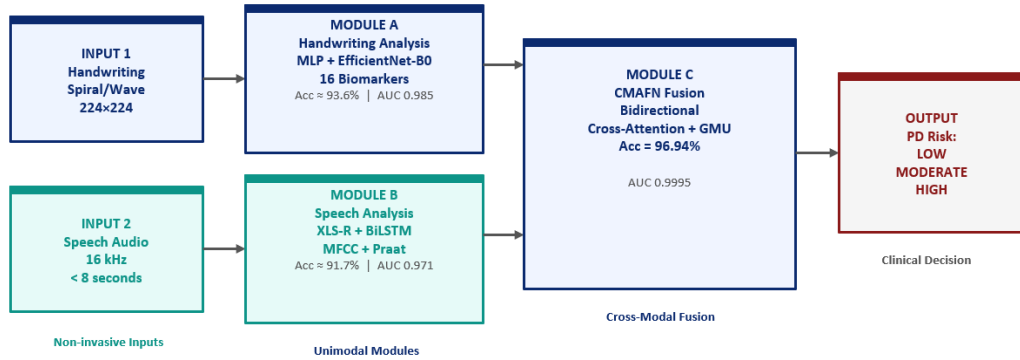
FIGURE 3: Proposed multimodal PD detection system with cross-modal fusion.
