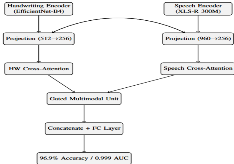
Figure 4.3: CMAFN architecture with cross-modal attention fusion of handwriting and speech achieving 96.9% accuracy and 0.999 AUC.
