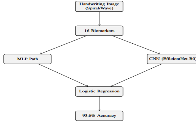
Figure 4.2.1: Dual-pathway handwriting analysis architecture combining Residual MLP and EfficientNet-B0 with meta-stacking.
