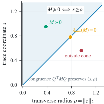
(b) Exact PSD--Lorentz geometry
