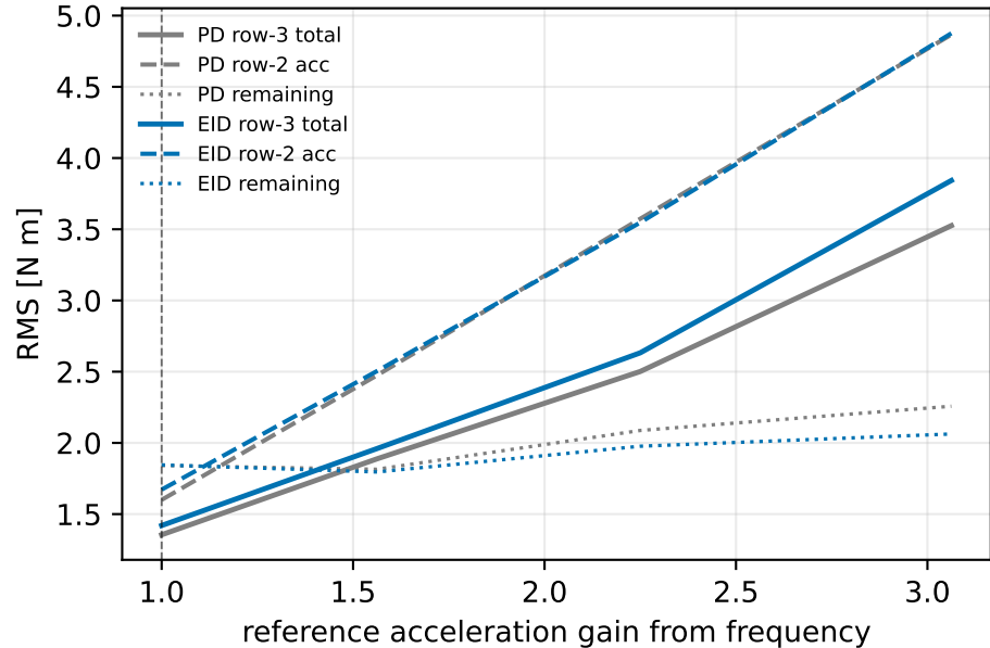
Knee acceleration -> hip residual
