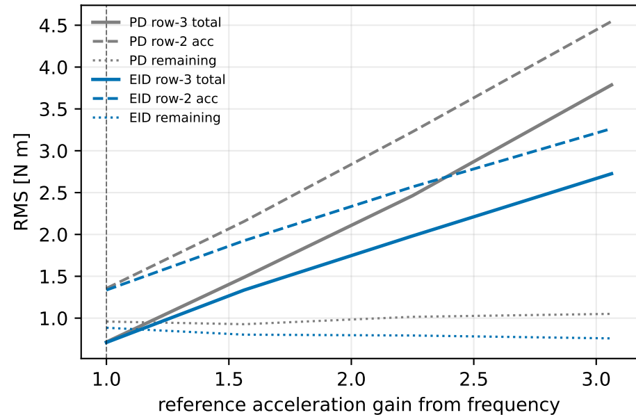
Hip acceleration -> knee residual
