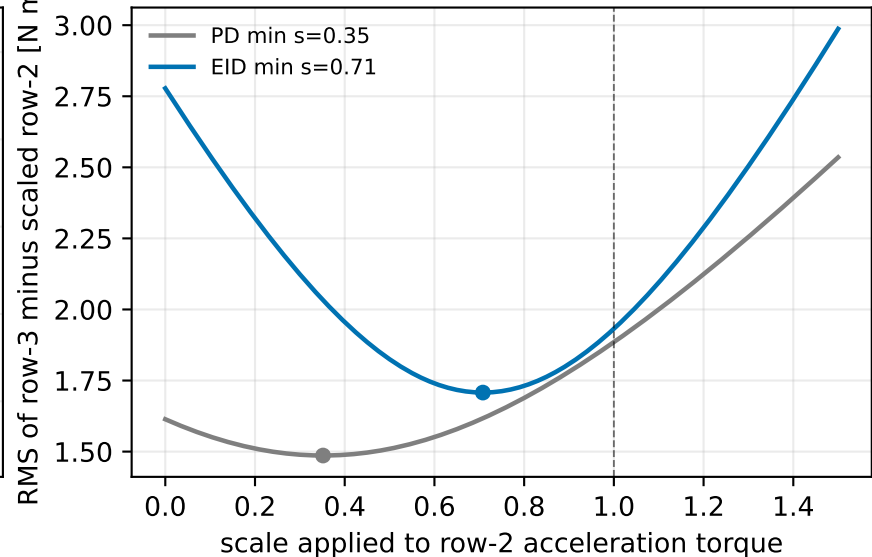
Knee acceleration term -> hip residual
