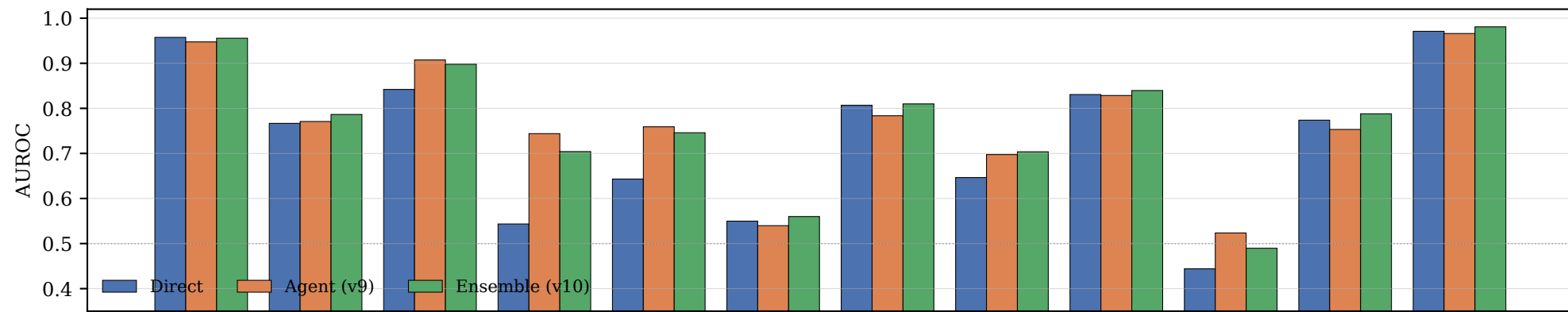
GPT-5.4 — Direct 0.731 / v9 0.768 / Ens 0.772 ( \Delta\text{Ens-Direct} = +4.01 pp, 95\%CI [+2.58, +5.50]★)
