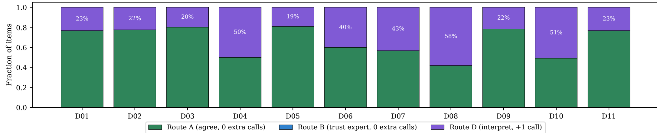
AnomalyClaw routing on SeedVL test (overall: A 67% / B 0% / D 33%; 1.33 VLM calls/img)
