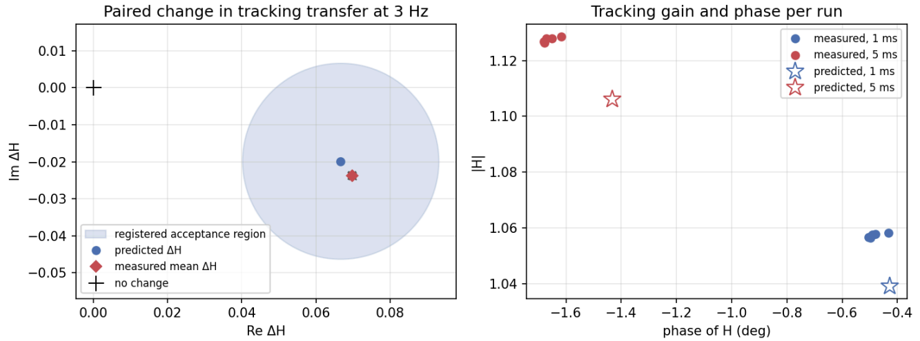
Figure 10. Prospective Task 5 test. Registered prediction and acceptance region (committed before the runs) against the five measured paired changes and their mean (the five pairs agree within 0.0003 and are hidden under the mean marker); right, per-run gain and phase with the predicted values. Simulated.
