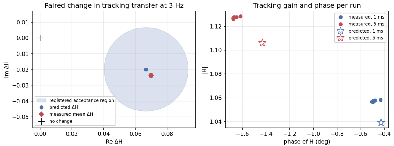
Figure 10. Prospective Task 5 test. Registered prediction and acceptance region (committed before the runs) against the five measured paired changes and their mean; right, per-run gain and phase with the predicted values. Simulated.
