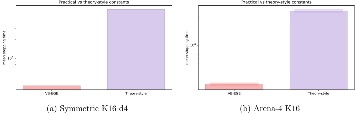
Figure 3: Paper and conservative constants on small instances. Darker overlays span mean \pm one standard error; the (8, 16, 4) sensitivity profile is deliberately more conservative.
