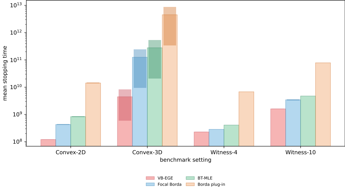
Figure 8: Convex and witness benchmark stopping times. Darker overlays show mean \pm one standard error.
