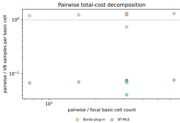
(a) Scaling tasks
