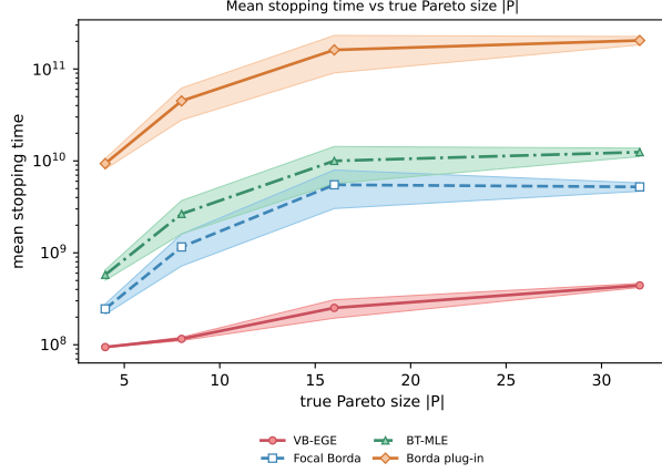
(a) Arena-4 tau
