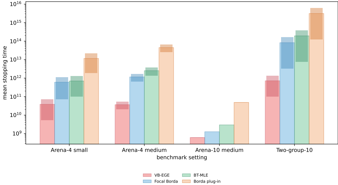
Figure 9: Arena and two-group benchmark stopping times. Darker overlays show mean \pm one standard error.
