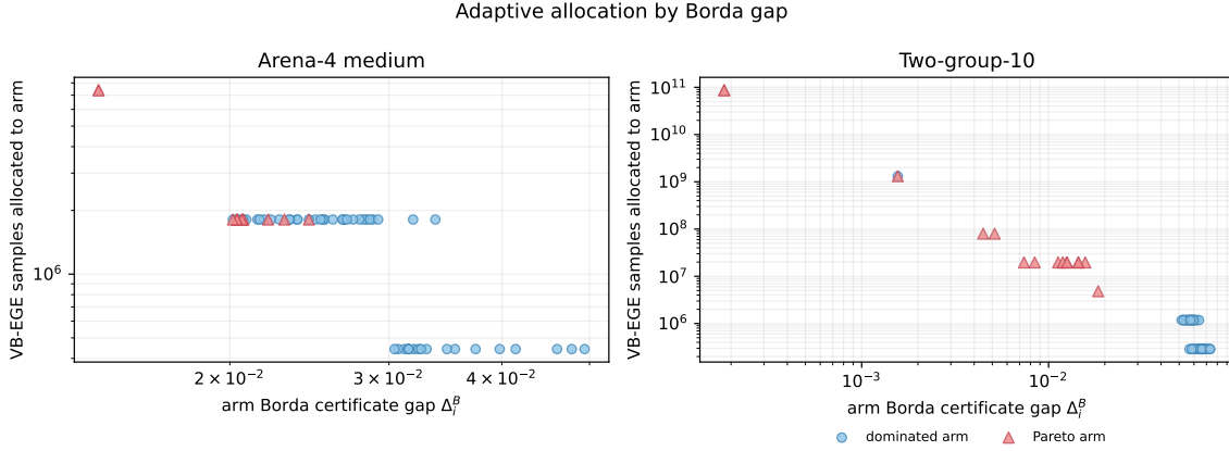
Figure 12: Arm allocation versus Borda certificate gap. Smaller-gap arms receive more VB-EGE samples in the representative runs.
