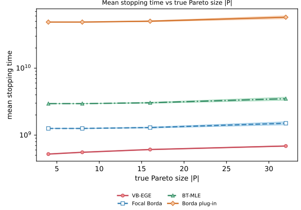
(b) Arena-10 tau
