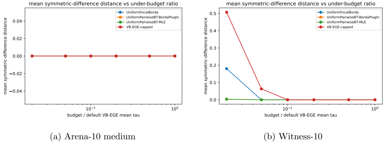
Figure 15: Under-budget Hamming-distance curves. The y-axis is mean symmetric-difference distance between the estimated and true Pareto sets.
