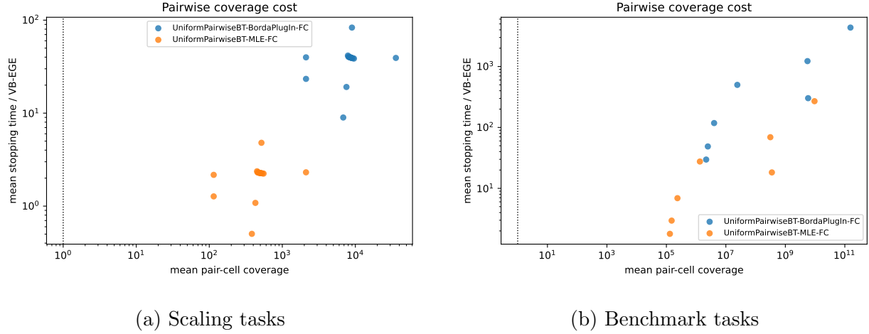
Figure 13: Pair-cell coverage cost diagnostics. Only pairwise baselines appear. The x-axis is total sampled pair-coordinate cells divided by dK(K-1)/2 ; the y-axis is mean stopping time divided by VB-EGE on the same setting.
