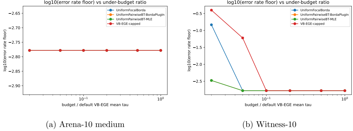
Figure 14: Under-budget empirical error curves. The x-axis is T/\bar{\tau}_{\text{VB,ref}} ; the y-axis is \log_{10} empirical error with the finite-sample floor only used when a method has no observed failures.
