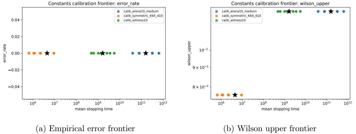
Figure 7: Calibration frontiers. Points near the lower-left are better only if their error remains below the target confidence level.
