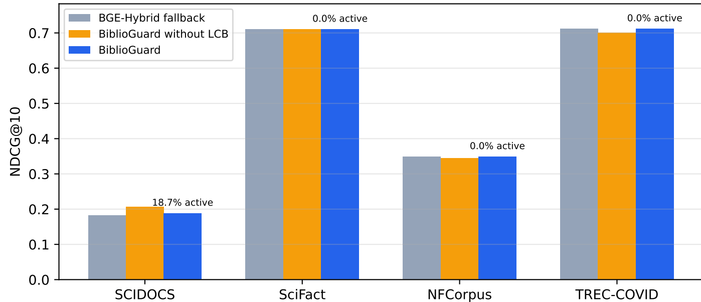
Confidence gating avoids observed cross-domain negative transfer
