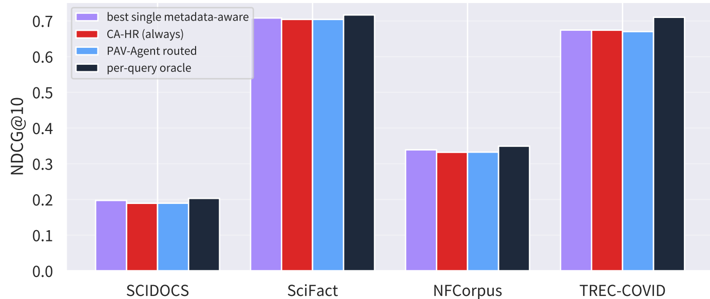
Oracle headroom vs. learned routing (NDCG@10)
