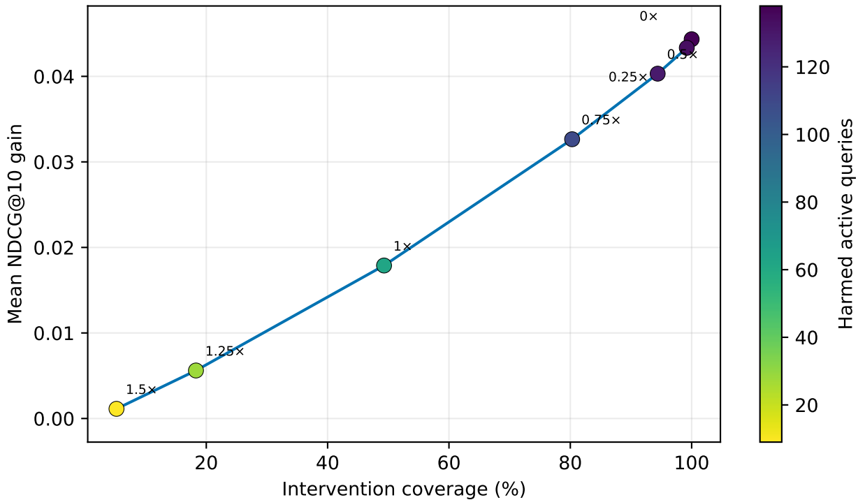
SCIDOCs risk-coverage trade-off
