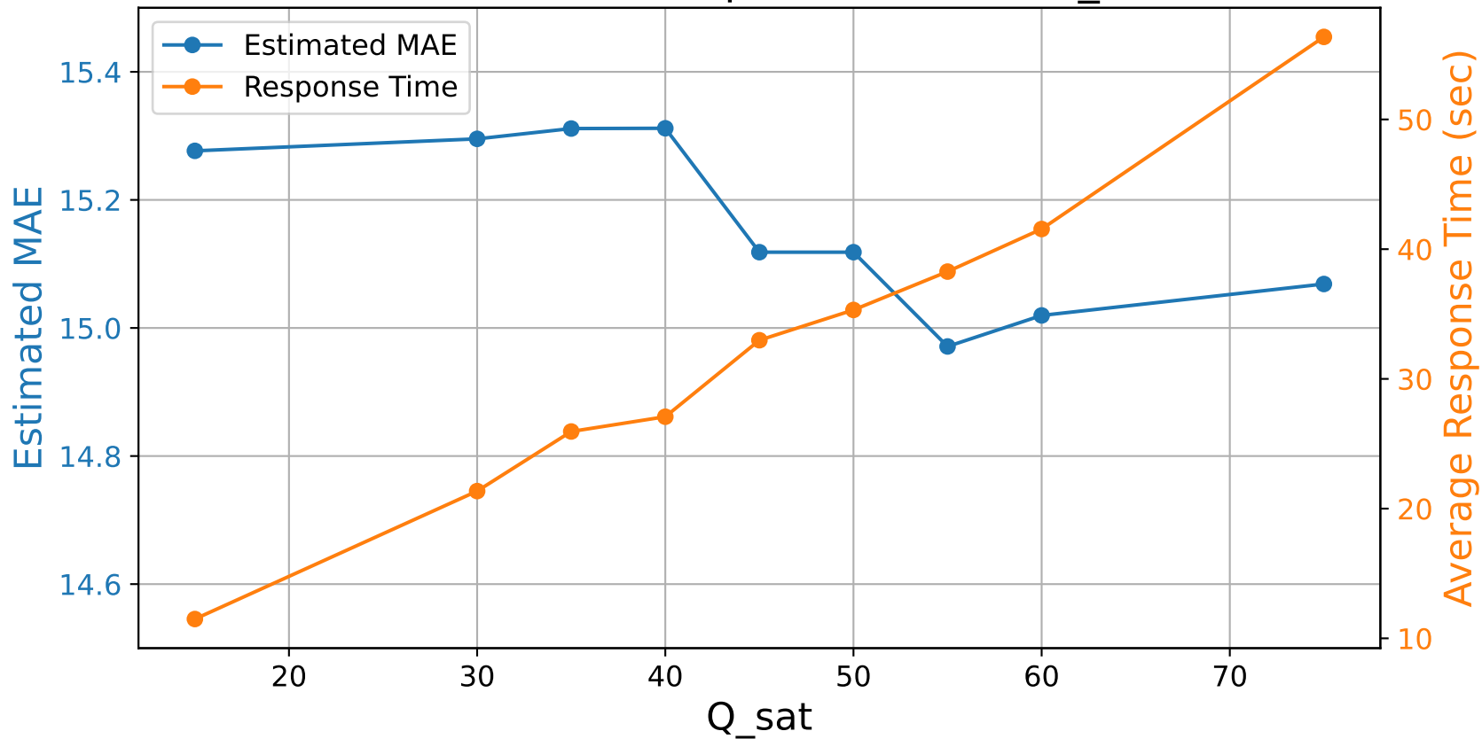
Estimated MAE and Response Time vs Q_sat ( \lambda=1 )
