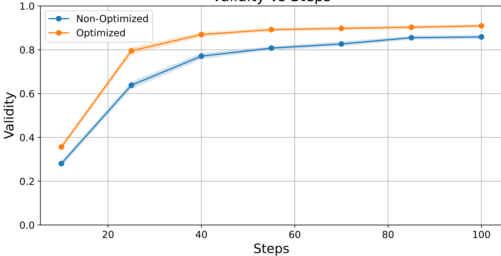
Validity vs Steps
