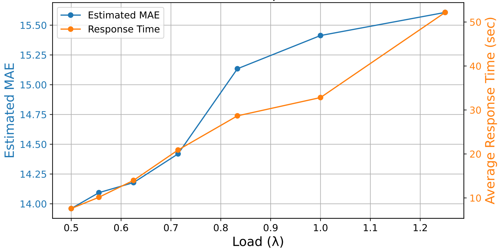
Estimated MAE and Response Time vs Load
