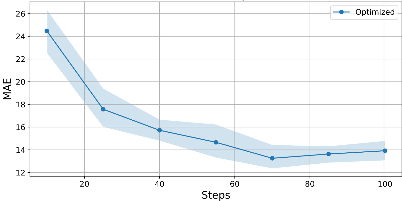
MAE vs Steps
