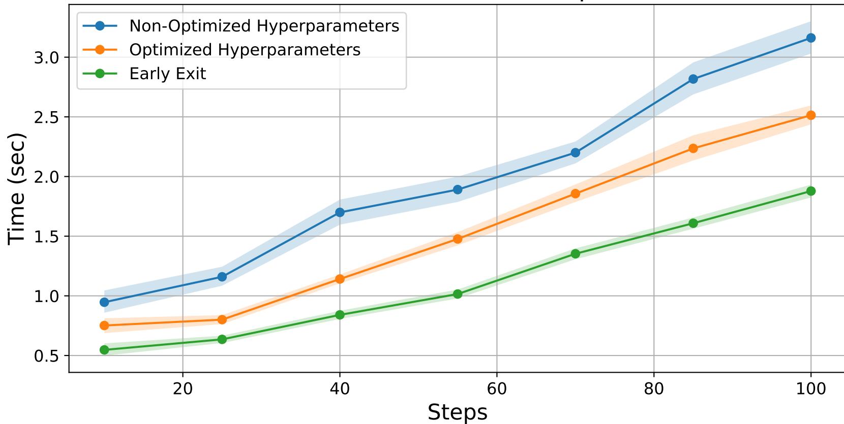
Execution Time vs Steps
