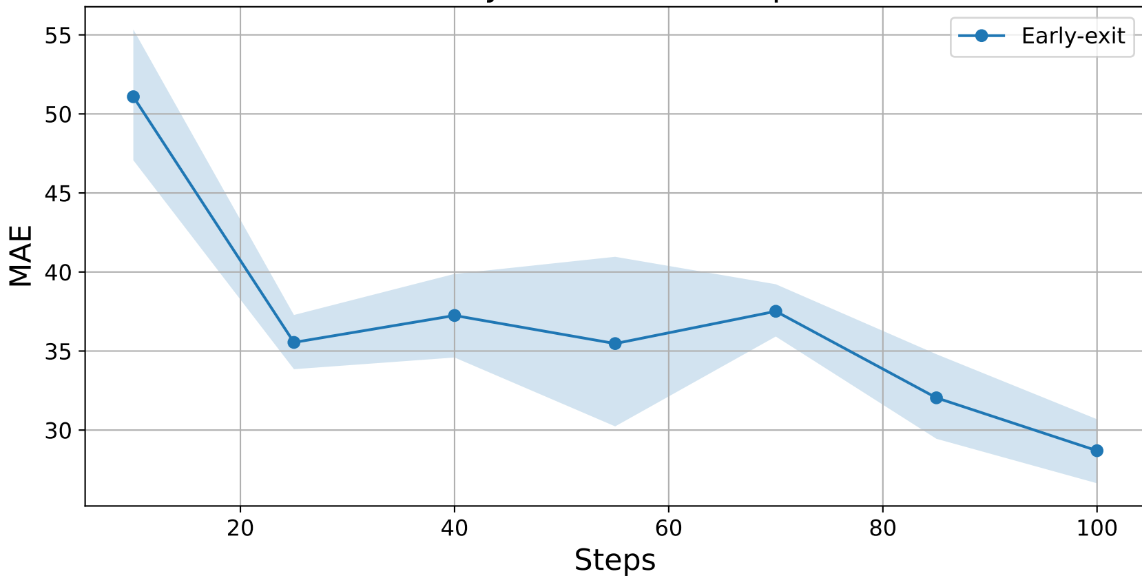
Early Exit MAE vs Steps
