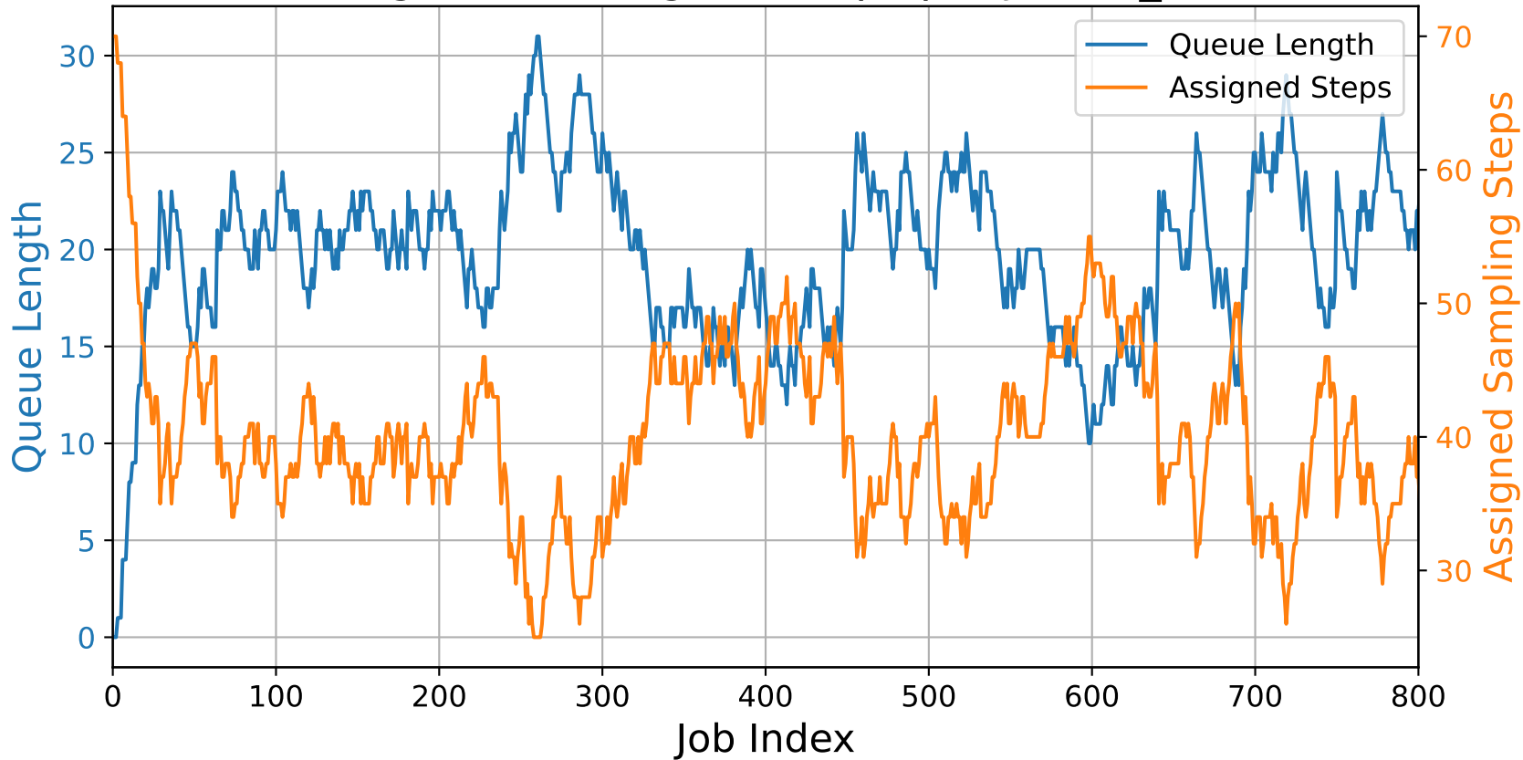
Queue Length and Assigned Steps per Job (Q_sat=30.0)
