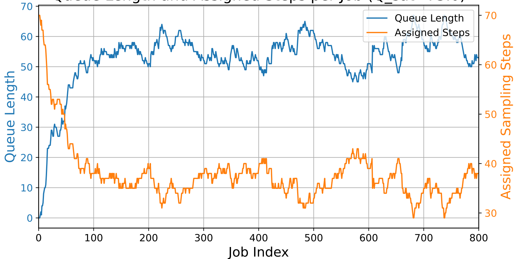
Queue Length and Assigned Steps per Job ( Q_{sat}=75.0 )
