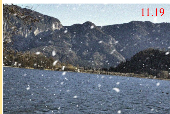
Input Image
