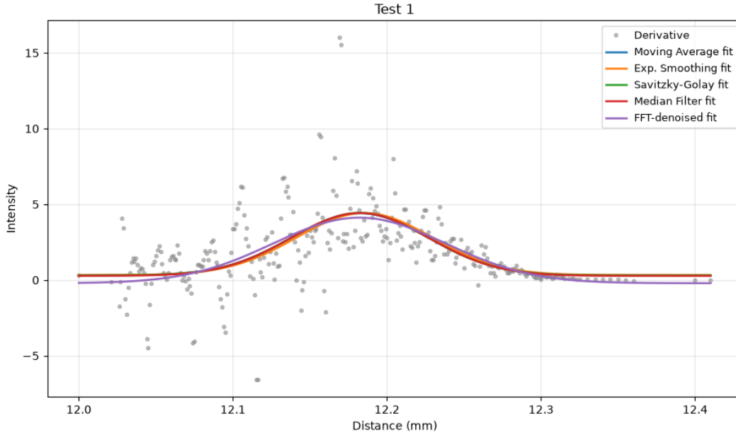
Figure 2: Final beam profile and Gaussian fits for Test 1.
