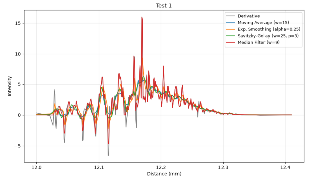
Figure 9: Test 1: Derivatives of standard smoothing outputs.
