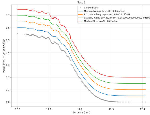
Figure 8: Test 1: Smoothed power curves (offset for clarity).
