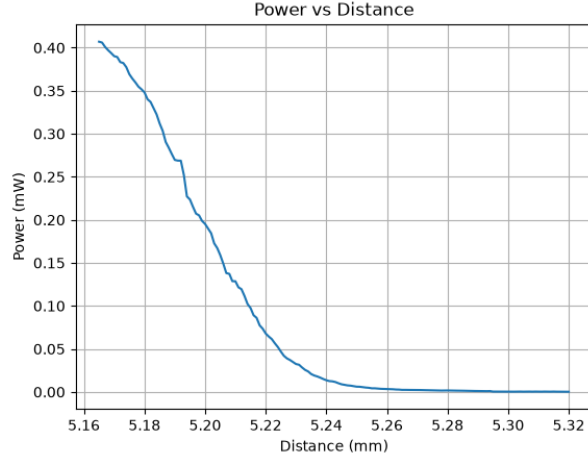
Figure 12: Test 2: Raw Power vs. Distance.
