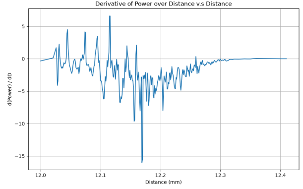
Figure 7: Test 1: Raw spatial derivative \frac{dP}{dD} .
