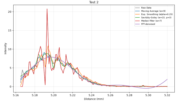
Figure 17: Test 2: FFT-denoised signal vs. standard smoothing.
