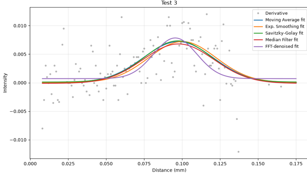
Figure 5: Final beam profile and Gaussian fits for Test 3 Filtered.
