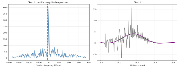
Figure 10: Test 1: Magnitude spectrum and spatial FFT filter.
