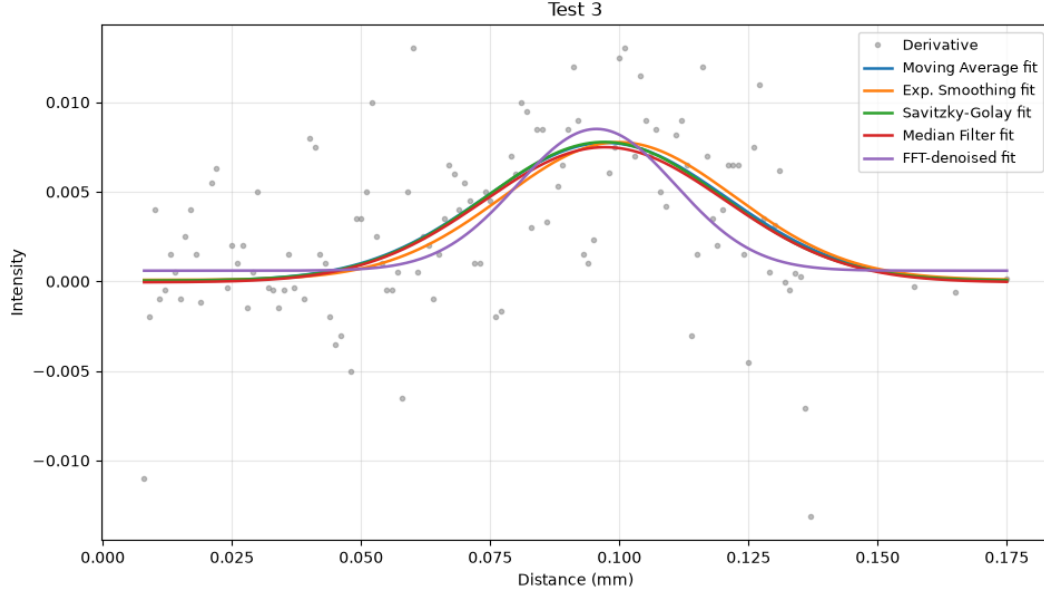
Figure 4: Final beam profile and Gaussian fits for Test 3.
