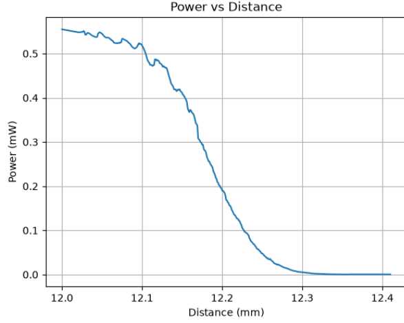
Figure 6: Test 1: Raw Power vs. Distance.
