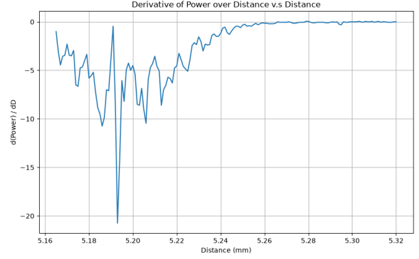
Figure 13: Test 2: Raw spatial derivative \frac{dP}{dD} .
