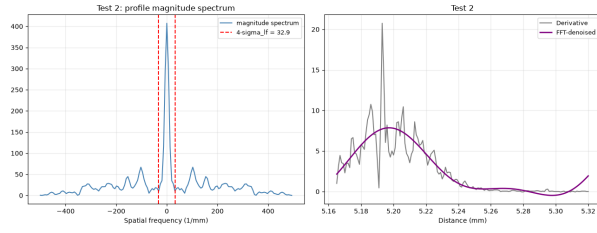
Figure 16: Test 2: Magnitude spectrum and spatial FFT filter.
