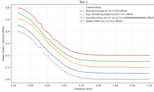
Figure 14: Test 2: Smoothed power curves (offset for clarity).
