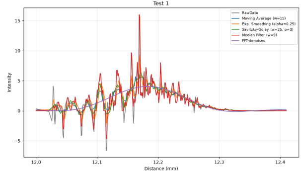
Figure 11: Test 1: FFT-denoised signal vs. standard smoothing.
