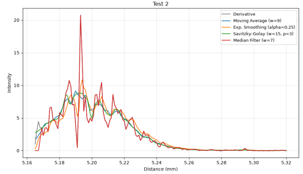
Figure 15: Test 2: Derivatives of standard smoothing outputs.
