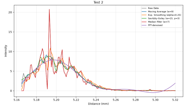
Figure 17: Test 2: FFT-denoised signal vs. standard smoothing.
