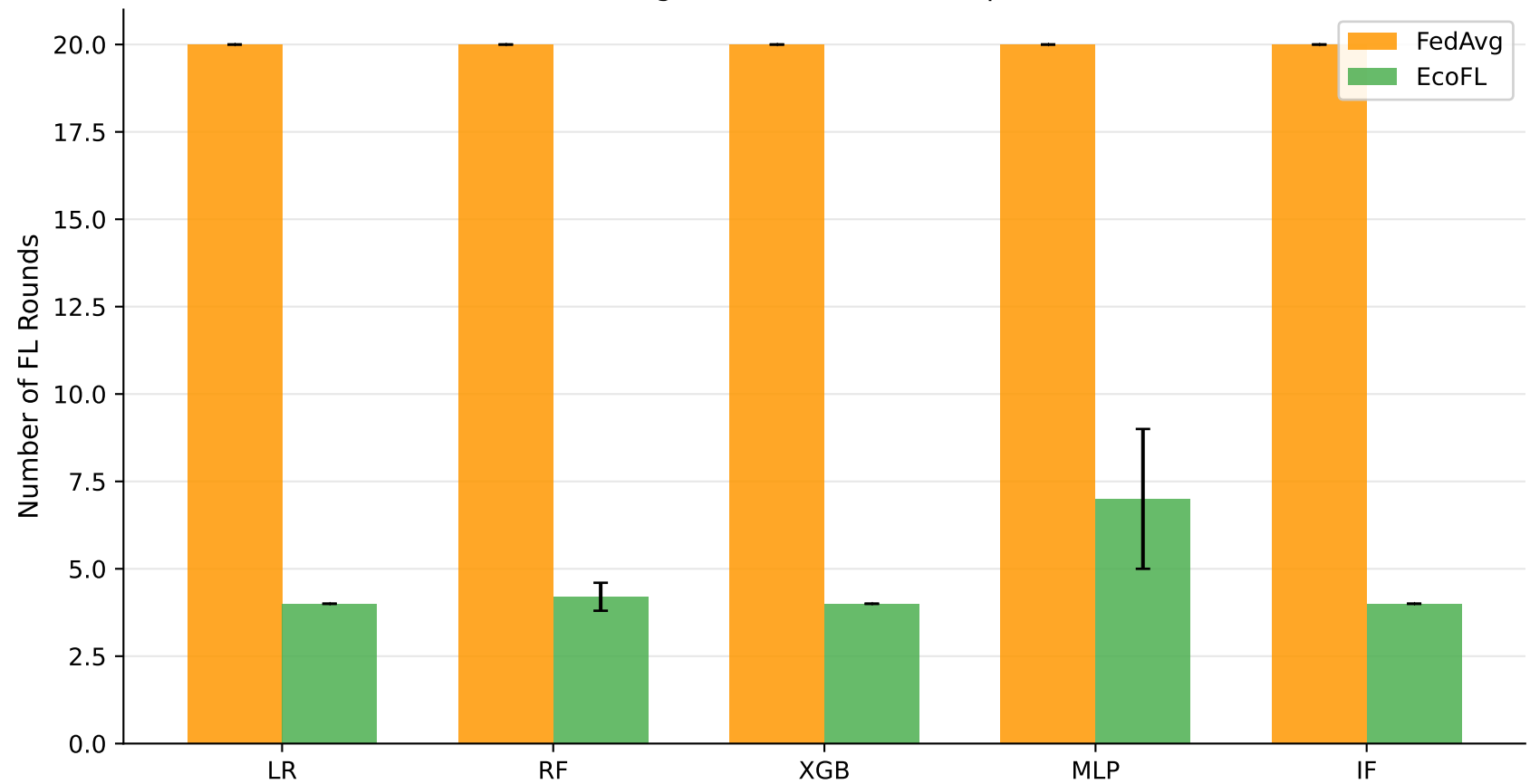
FL Rounds: FedAvg (fixed) vs EcoFL (adaptive termination)
