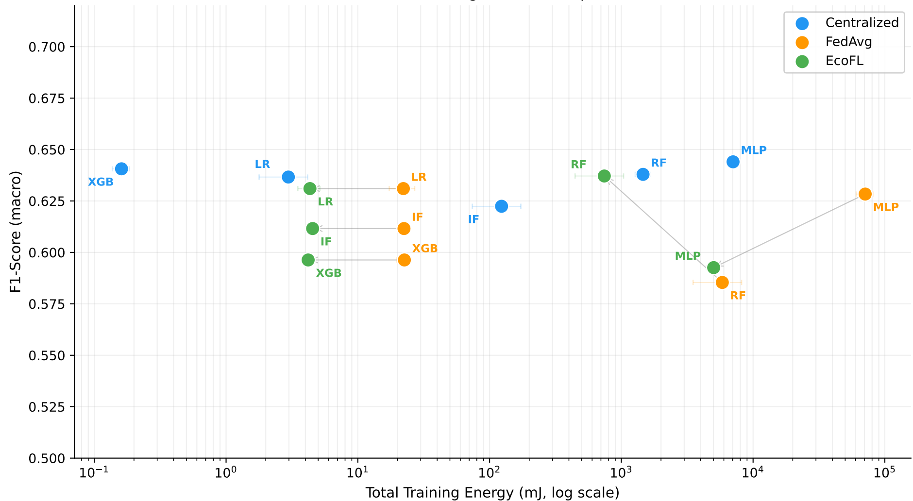
Pareto Frontier: F1-Score vs Training Energy (arrows show FedAvg → EcoFL shift per model)
