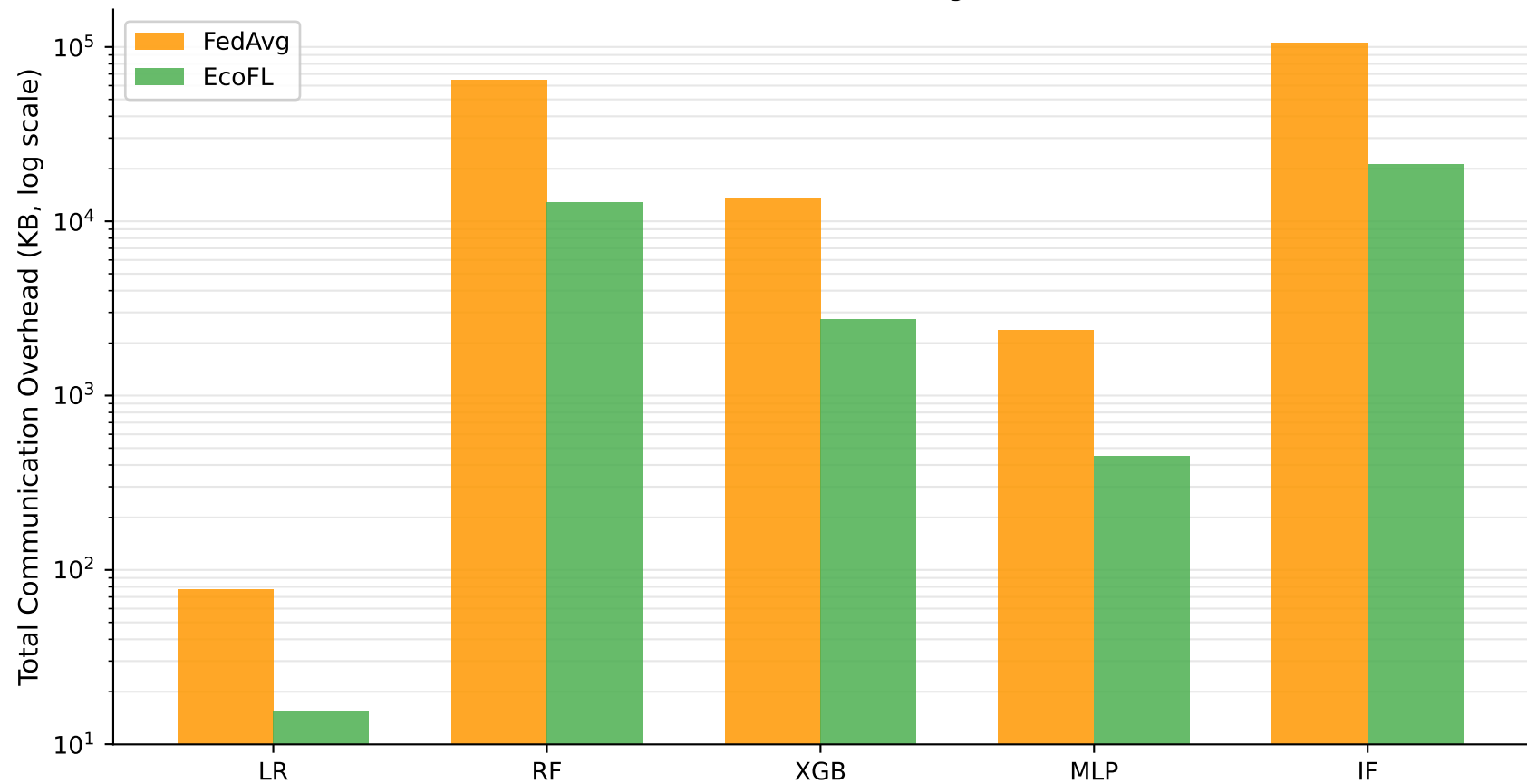
Communication Cost: FedAvg vs EcoFL
